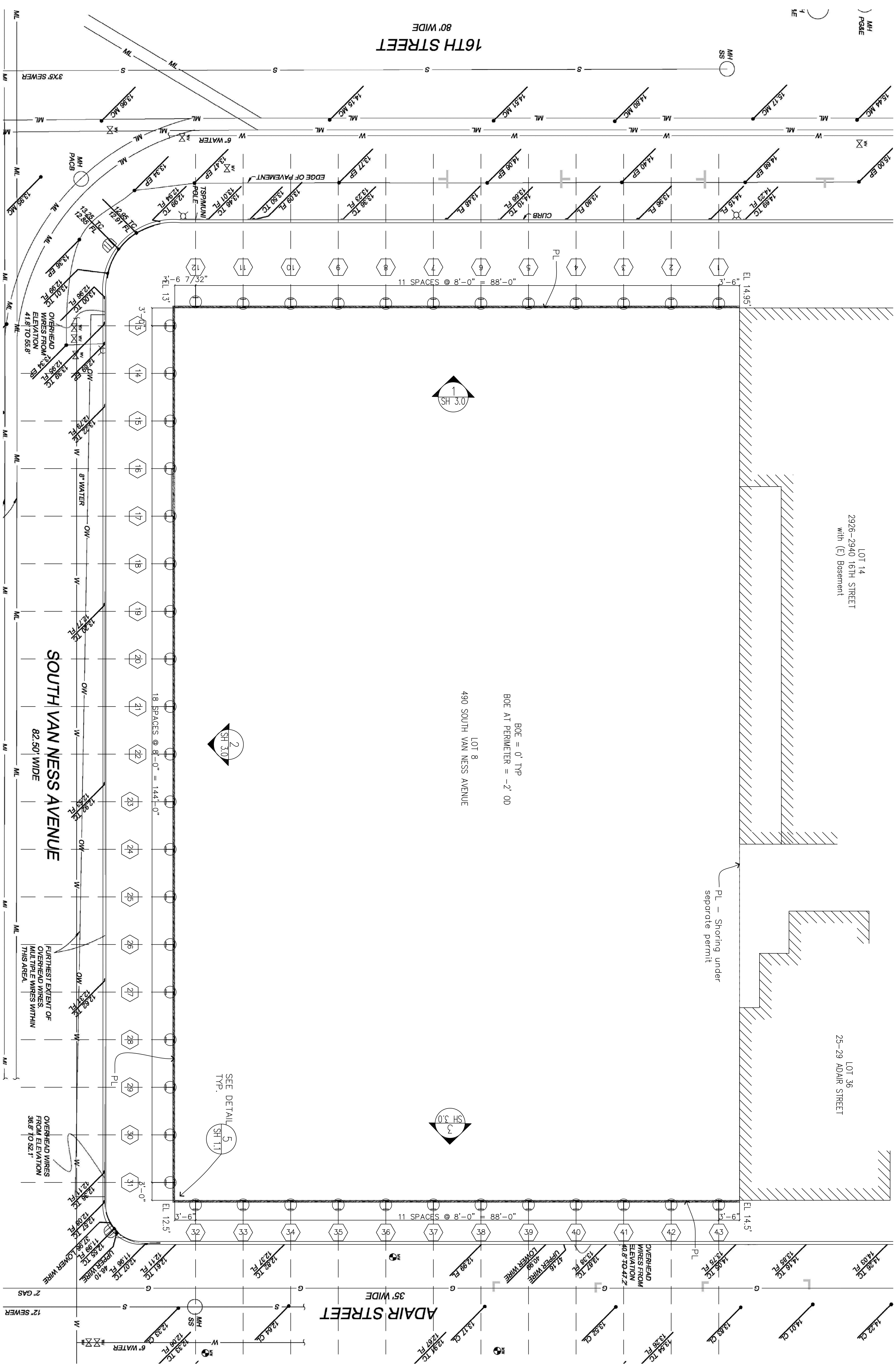
1 SHORING PLAN SH 2.0 SCALE: 1/8" = 1'-0"
