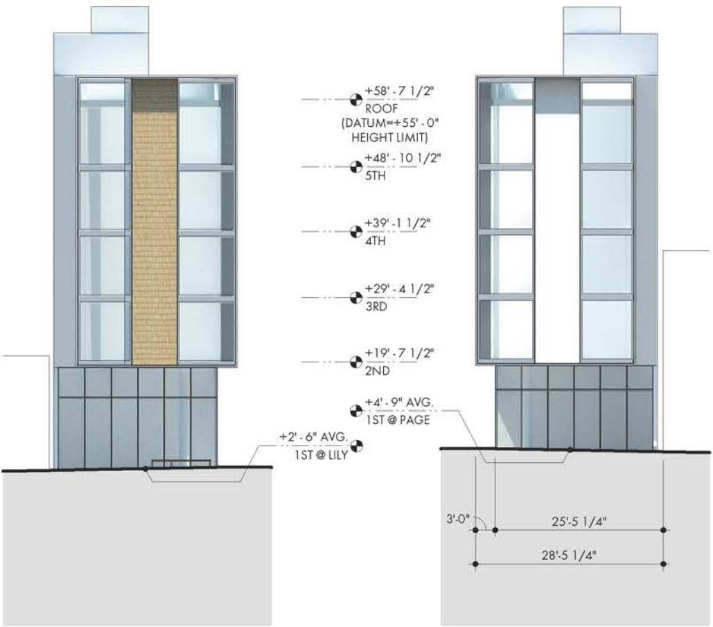
NORTH ELEVATION
