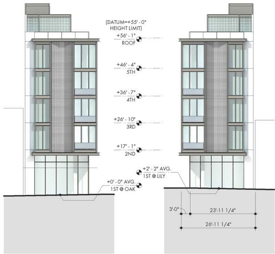
NORTH ELEVATION
